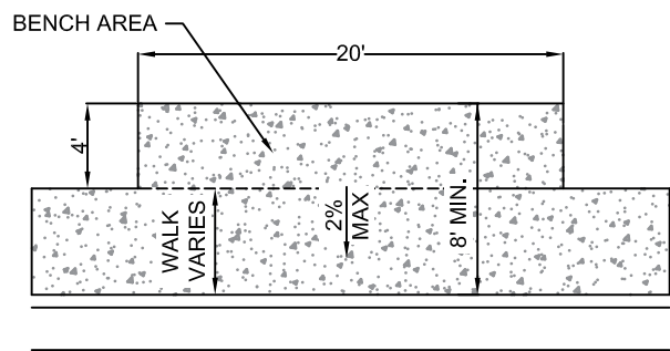
ATTACHED WALK BENCH PAD
