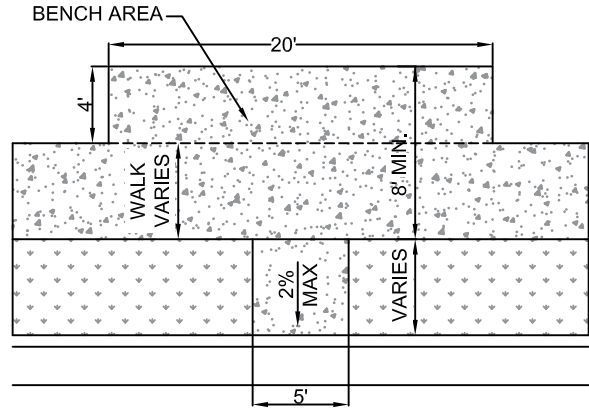
DETACHED WALK BENCH PAD AND CONNECTION
