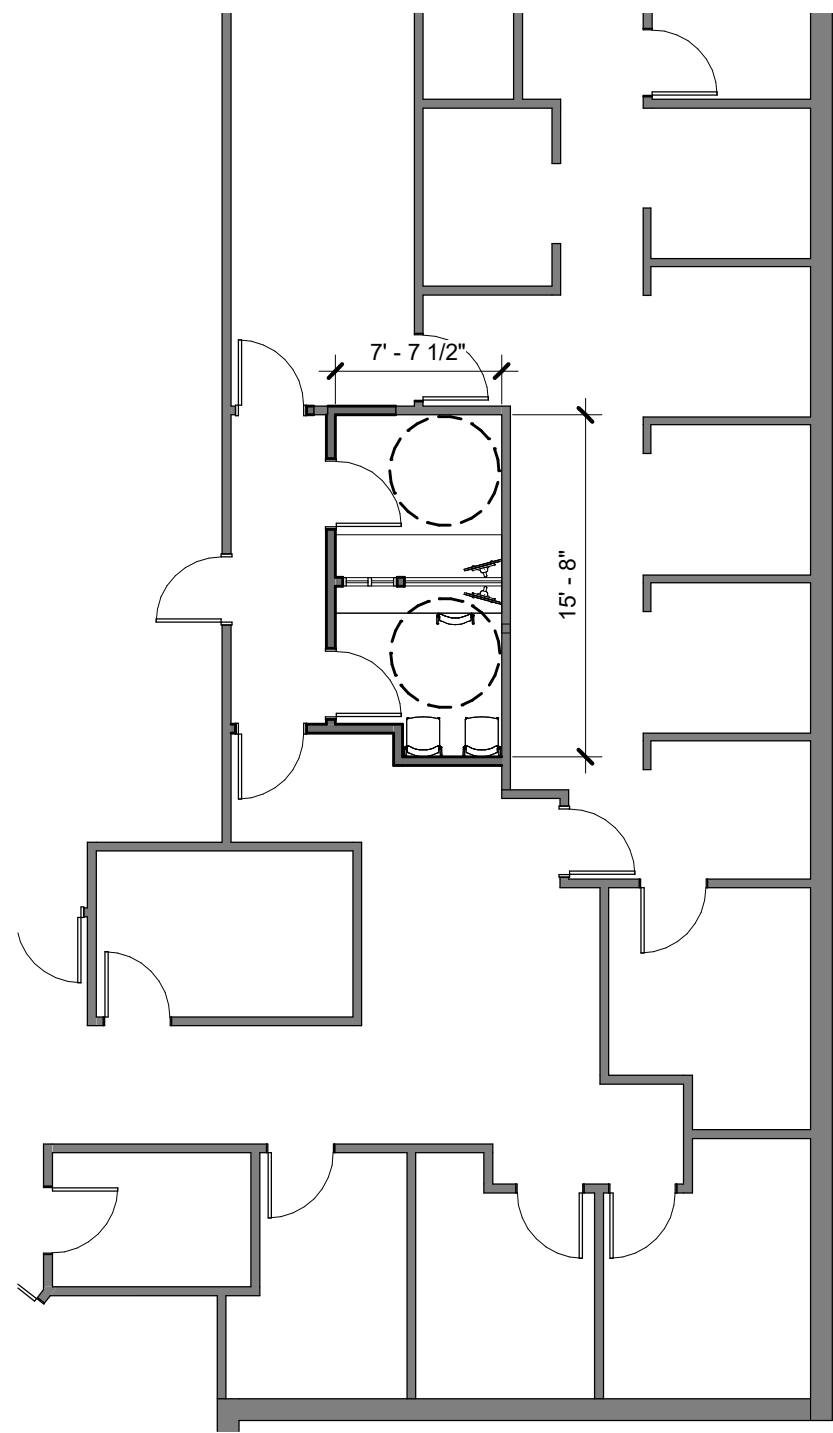
1 A983 OPTION 1 - COURT 1/8" = 1'-0"
