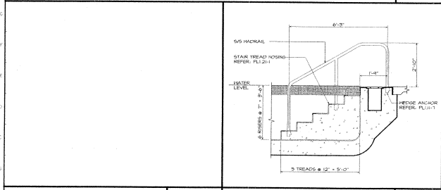
STAIR SECTION
